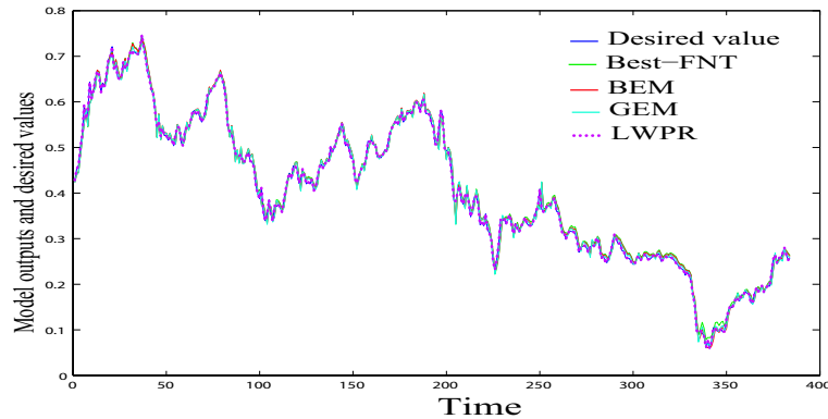
Fig. 3. Test results showing the performance of the different methods for modeling the NIFTY index
